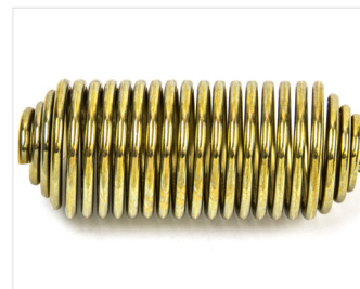
SH8 Maximum diameter: 1-1/4" Length: 3-1/8" Fit: 1/2" rod or custom
