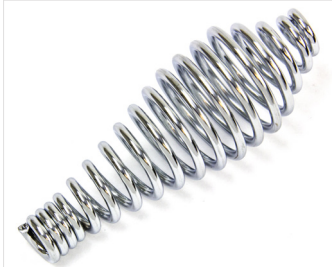
SH2 Maximum diameter: 1-1/2" Length: 4-1/4" Fit: 1/2" rod or custom
