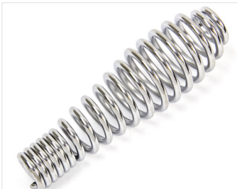
SH10 Maximum diameter: 1-1/4" Length: 4-1/4" Fit: 1/2" rod or custom
